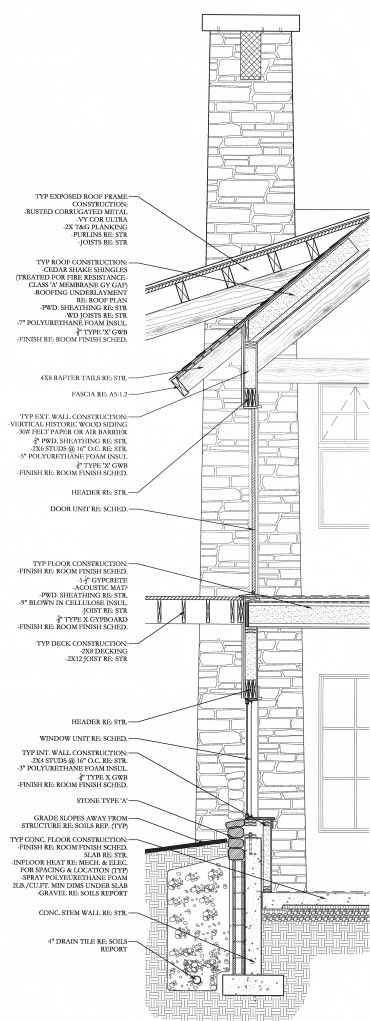
6 WALL SECTION AT MASTER BEDROOM TYP - 1/4"
