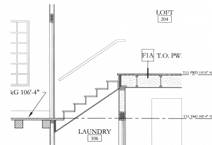
5 LOFT STAIR SECTION 10'-0" x 10'-0"
