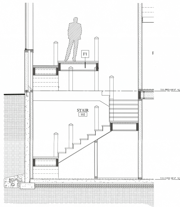
3 TOWER STAIR SECTION 10'-0" x 10'-0"
