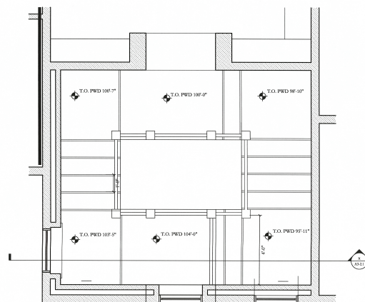
4 TOWER STAIR PLAN 10'-0" x 10'-0"
