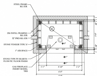
5 MASTER FIREPLACE LOWER PLAN
