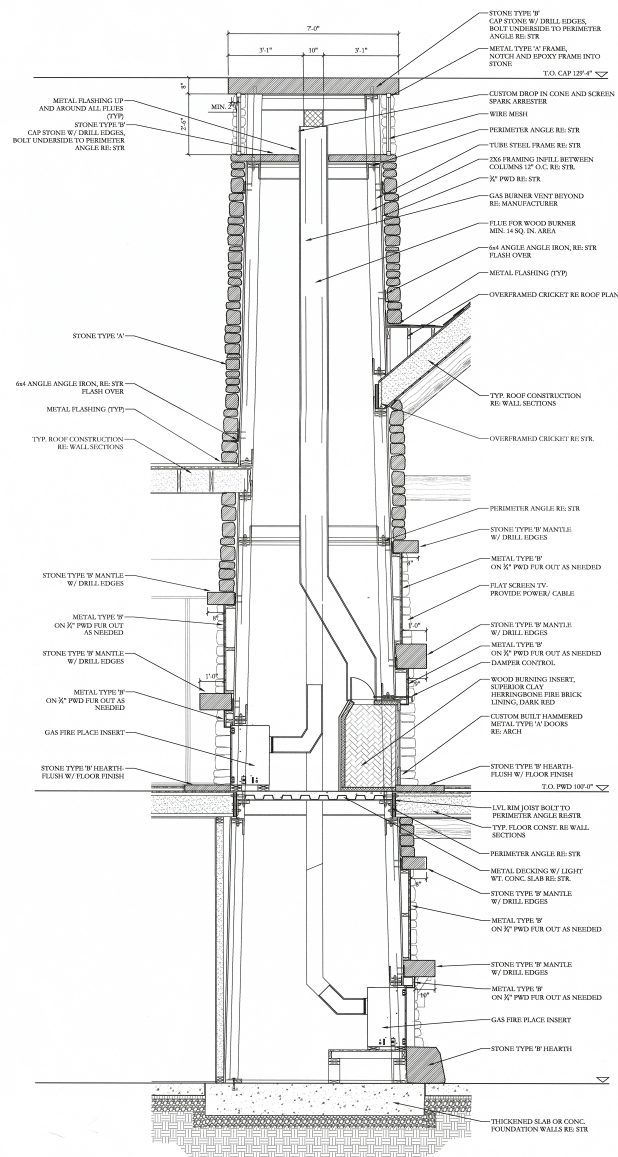
1 MAIN FIREPLACE SECTION 1/2" = 1'-0"
