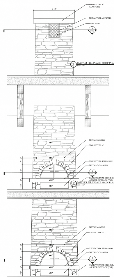
2 MASTER FIREPLACE ELEVATION
