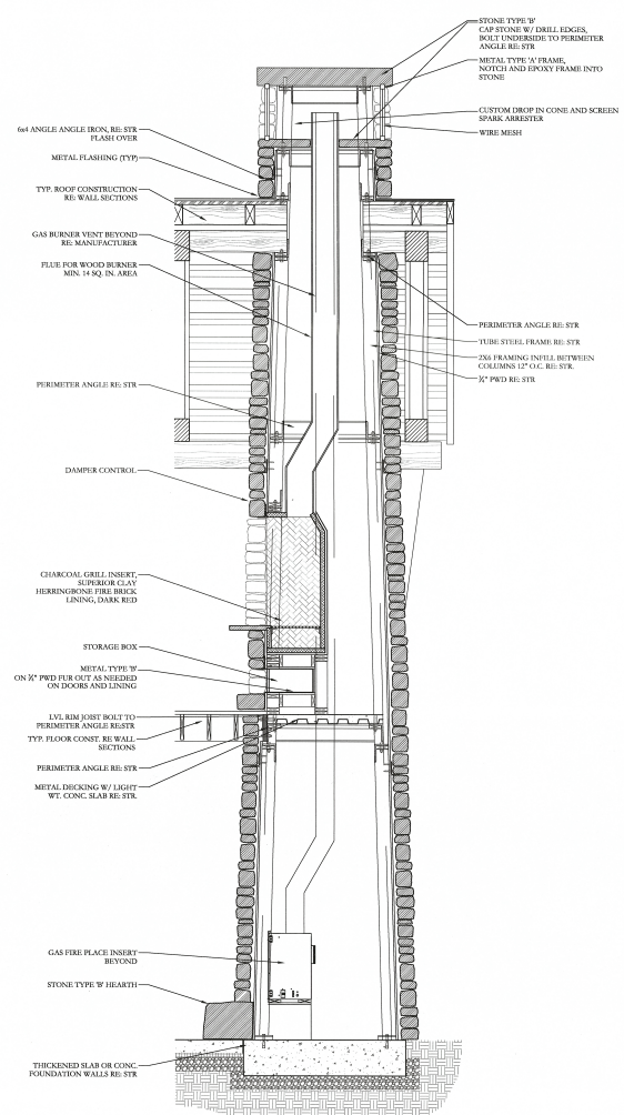
5 PATIO FIREPLACE SECTION 10'-7 1/4"
