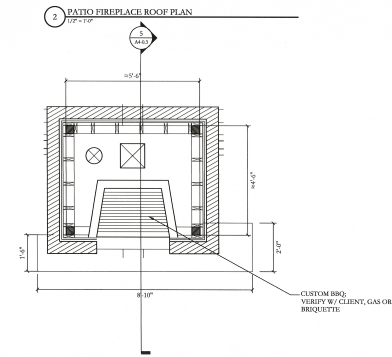
2 PATIO FIREPLACE ROOF PLAN 10'-7 1/4"
