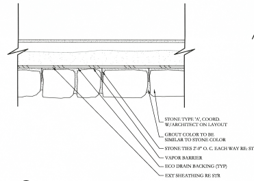
6 STONE PLAN DETAIL 1/2" = 1'-0"
