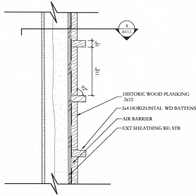
1 SIDING DETAIL 1/2" = 1'-0"
