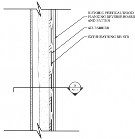
2 SIDING DETAIL 1/2" = 1'-0"
