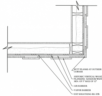
8 SIDING OUTSIDE CORNER DETAIL 1/2" = 1'-0"
