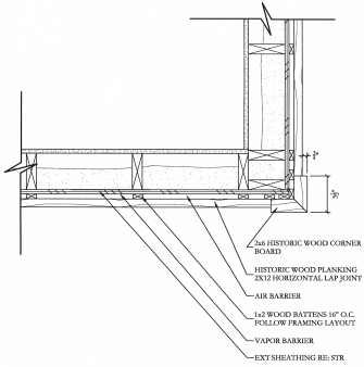
7 SIDING OUTSIDE CORNER DETAIL 1/2" = 1'-0"
