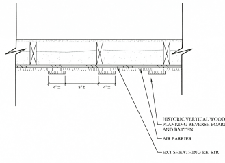
5 SIDING PLAN DETAIL 1/2" = 1'-0"
