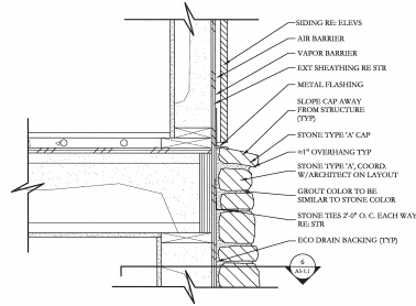
3 STONE CAP DETAIL 1/2" = 1'-0"
