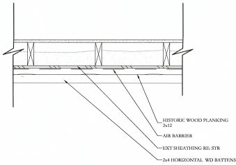
4 SIDING PLAN DETAIL 1/2" = 1'-0"
