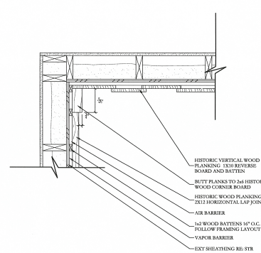
9 SIDING INSIDE CORNER DETAIL 1/2" = 1'-0"
