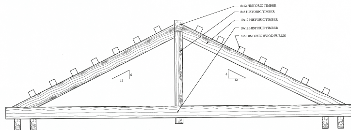
2 TRUSS TYPE 'B' TOP VIEW
