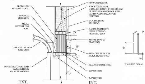
13 GARAGE DOOR HEAD AT SIDING 1 1/2\"/>
