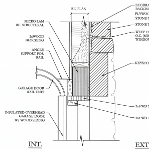
4 GARAGE DOOR HEAD AT STONE 1 1/2\"/>
