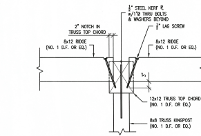
TIMBER RIDGE CONNECTION DETAIL 5 3/4" = 1'-0"
