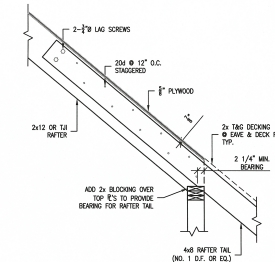
RAFTER TAIL CONNECTION DETAIL 9 3/4" = 1'-0"
