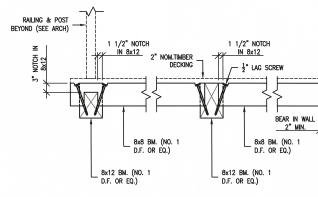
DECK SECTION 6 3/4" = 1'-0"
