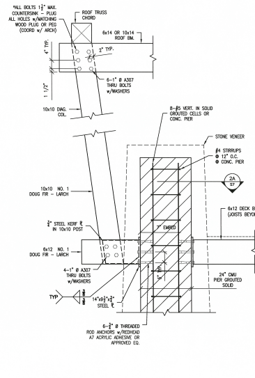
DECK SECTION 2 3/4" = 1'-0"
